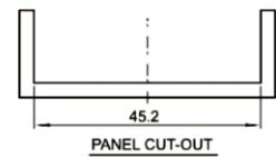
PANEL CUT-OUT
