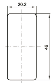
PANEL CUT-OUT
